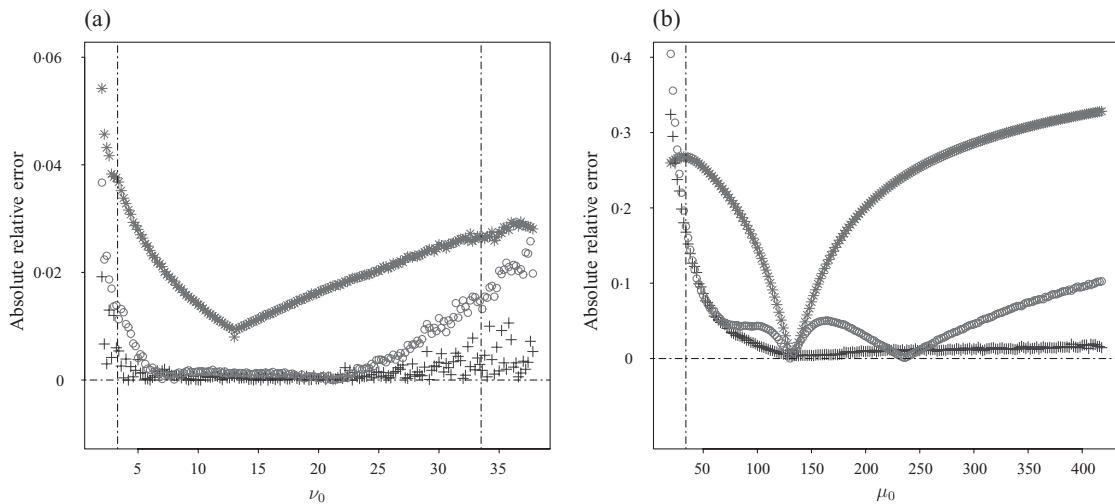
Fig. 2. Absolute relative errors of approximations of conditional p -values, (a) gamma shape example, (b) gamma mean example. Plots show results for bootstrap (1), +, bootstrap (5), o, \Phi(r) , x, and \Phi(r^*) , *.
