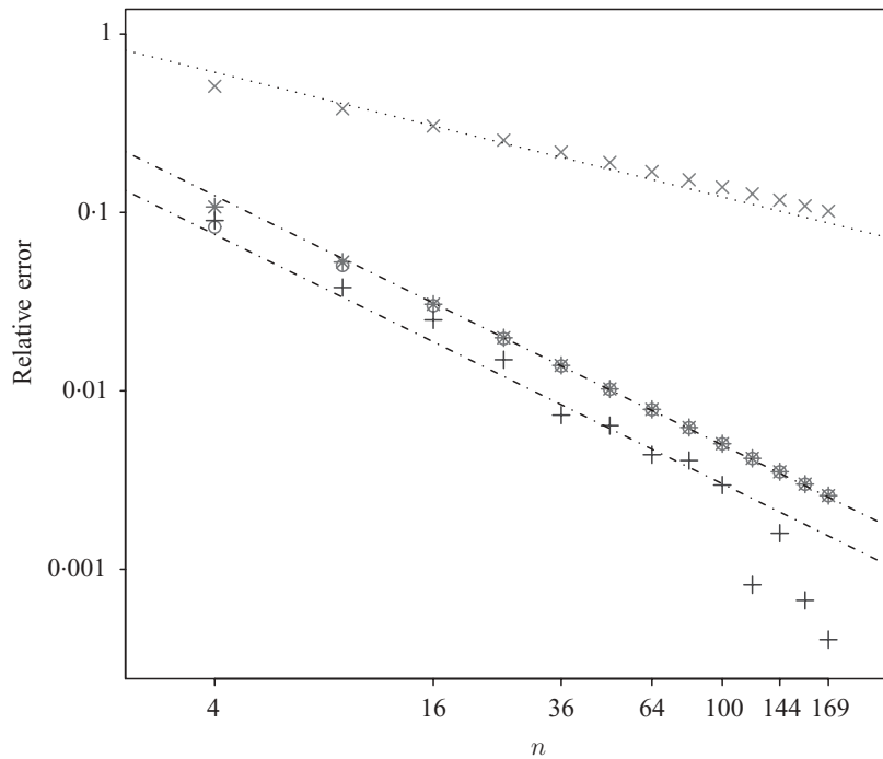
Fig. 3. Binomial example. Logarithmic plot of relative errors of approximations of conditional p -values against sample size n . Plots show results for bootstrap (1), +, bootstrap (5), o, \Phi(r) , x, and \Phi(r^*) , *.
