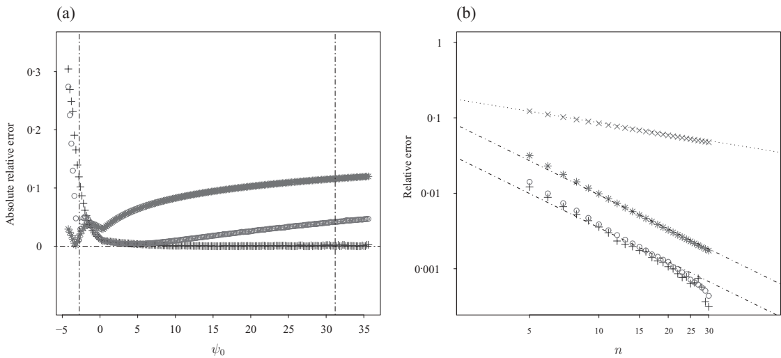
Fig. 1. Lognormal mean example. (a) Absolute relative errors of approximations of conditional p -values. (b) Logarithmic plot of relative errors of approximations against sample size n . Plots show results for bootstrap (1), +, bootstrap (5), \circ , \Phi(r) , \times , and \Phi(r^*) , * .
