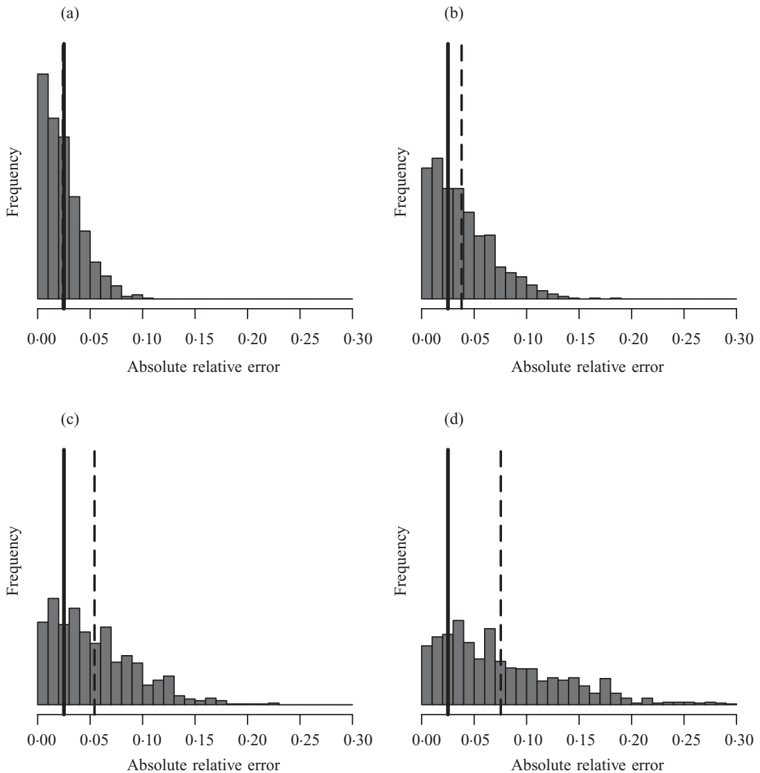
Fig. 4. Histogram of absolute relative errors of 1000 bootstrap estimators based on different simulation sizes B , testing gamma shape \nu = 30 . Solid vertical line indicates absolute relative error of analytic approximation \Phi(r^*) , broken vertical line the average of the 1000 bootstrap absolute relative errors. (a) B = 50\,000 , (b) B = 20\,000 , (c) B = 10\,000 , (d) B = 5000 .
