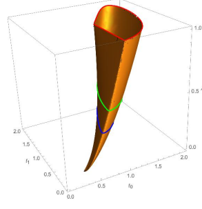
FIGURE 2. The moduli space \mathcal{M}
