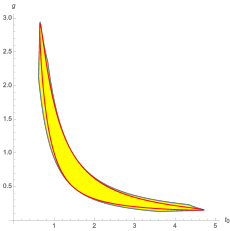
FIGURE 3. The curve C^* in S
