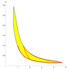
FIGURE 4. Folded C^* in \mathcal{M}
