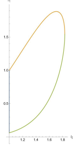
FIGURE 1. The level set S_1
