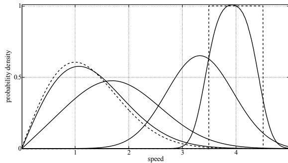
Figure 6: Evolution of an initial probability measure, \mu_0 , of the free mass velocity, having a step function density. The graphs in dashed line are the initial and the limit density v \exp(-v^2/2) , and the other graphs, from right to left, are the densities of \mu_0 P^n at steps n = 1, 10, 50, 100 , of the Markov chain of Proposition 5. We have used a finite rank approximation of P obtained by numerically simulating the mechanical system with mass ratio m_1/m_2 = 100 .
