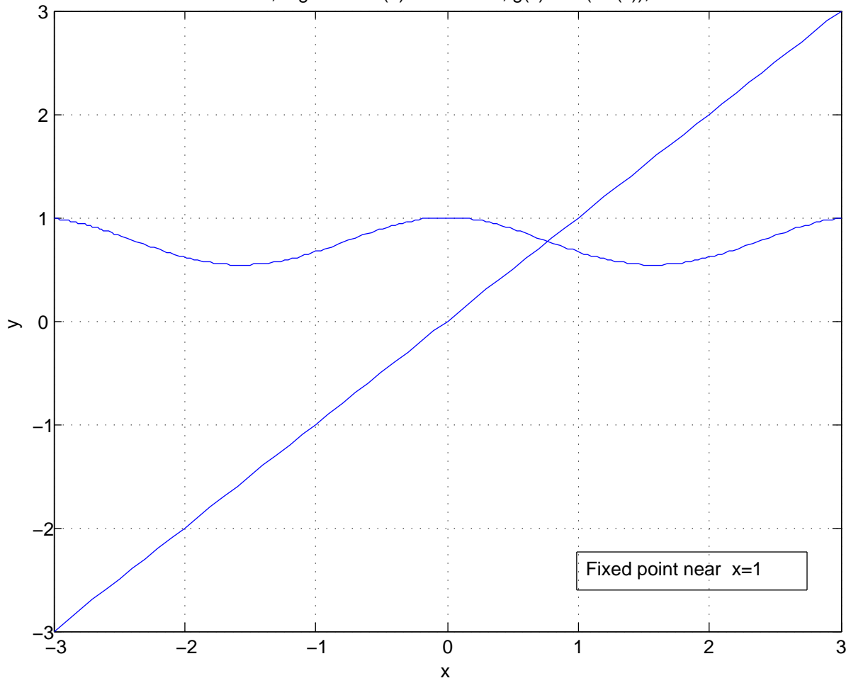
Homework 2, Algorithm 1 (b) section 2.1, g(x)=\cos(\sin(x)) , R. Feres
