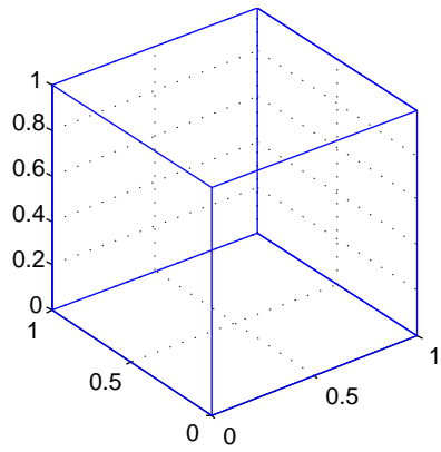
Initial position of the cube
