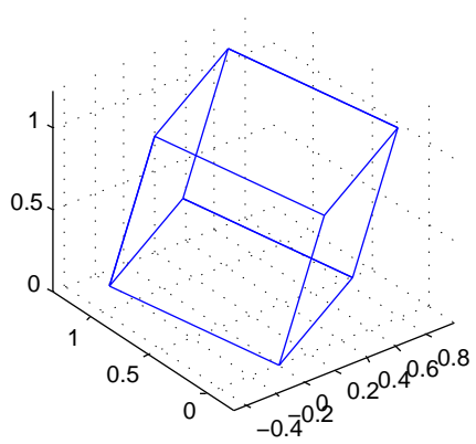
After rotation by R_z(\pi/6) * R_x(\pi/12)
