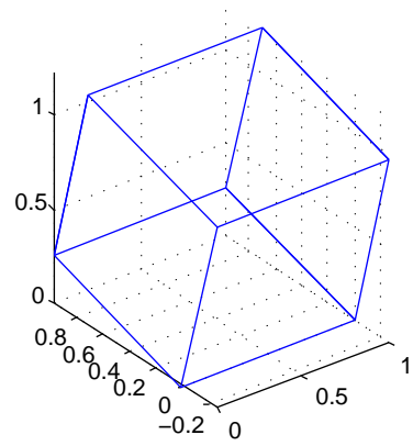
After rotation by R_x(\pi/12)
