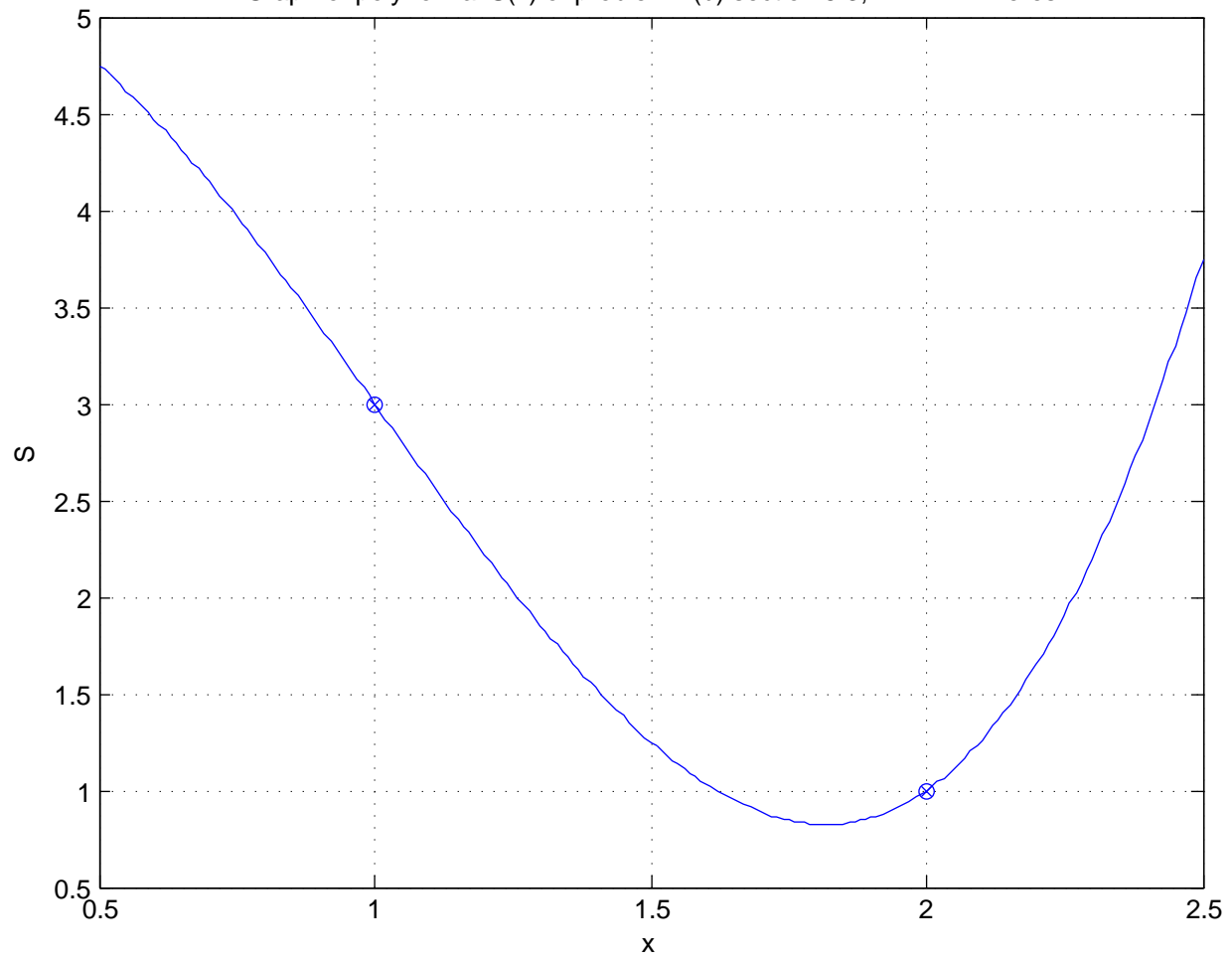
Graph of polynomial S(x) of problem 2(b) section 5.3, HW 7. R. Feres
