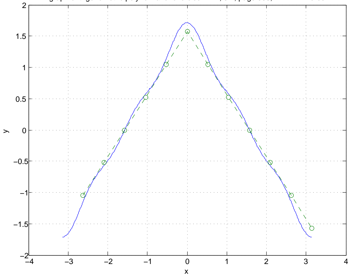
graph of trigonometric polynomial of exercise AP 1, 5.4, page 308, HW 7 R. Feres
