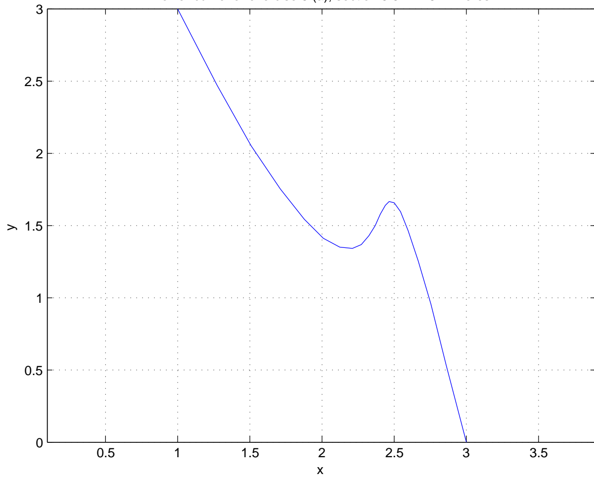
Bezier curve for exercise 8 (a), section 5.5 HW 8 R. Feres
