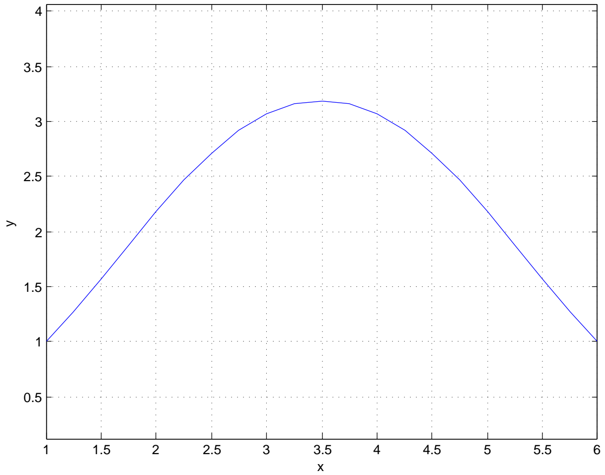
Bezier curve for Exercise 8 (c), section 5.5 HW 8 R. Feres
