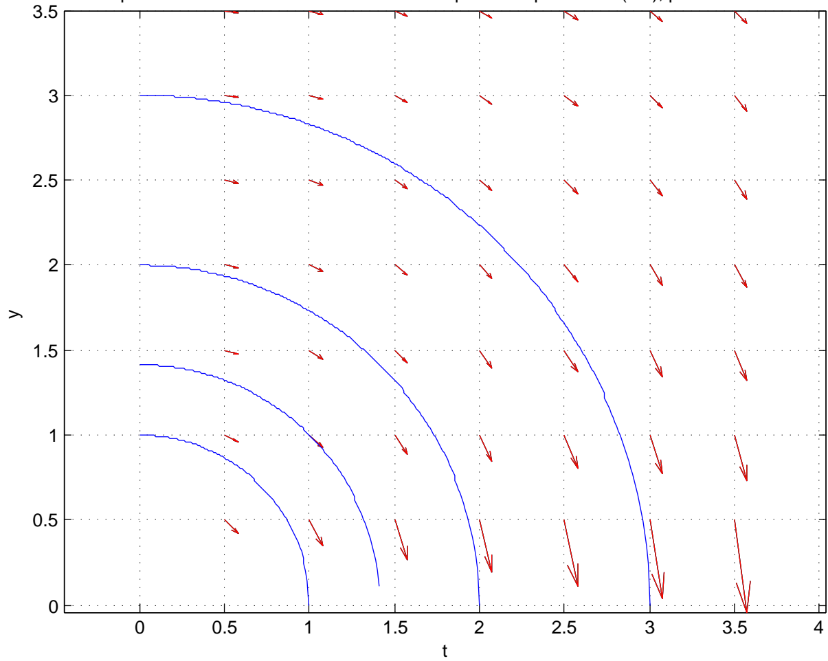
Slope field and solutions to the differential equation of problem 6 (9.1), p. 462. R. Feres
