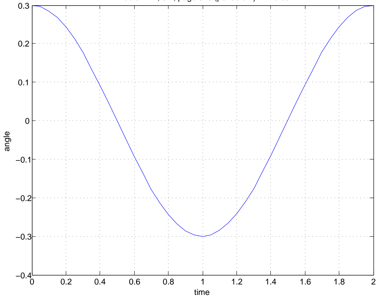
Problem 12, 9.7, page 526 (pendulum) R. Feres
