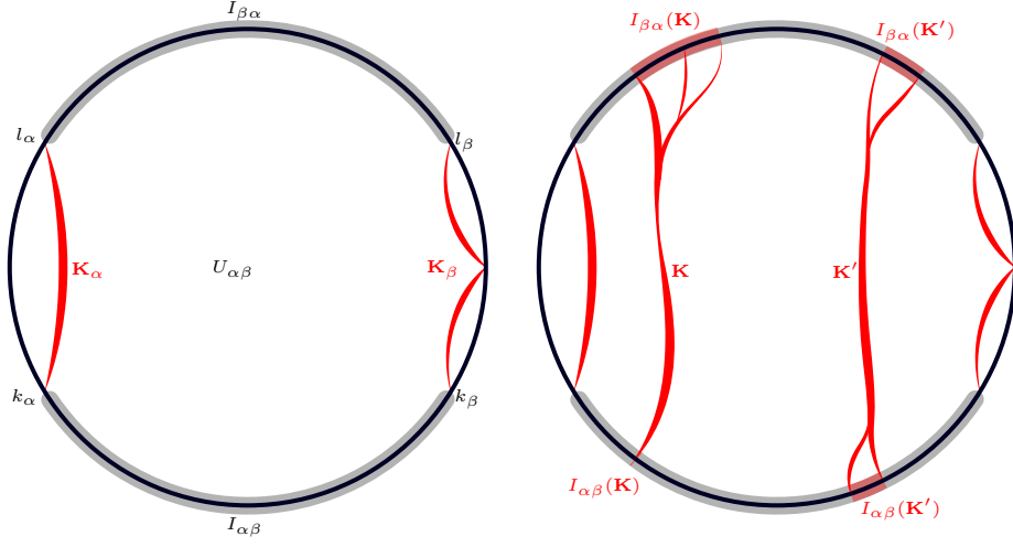
FIGURE 7. The separation interval.
